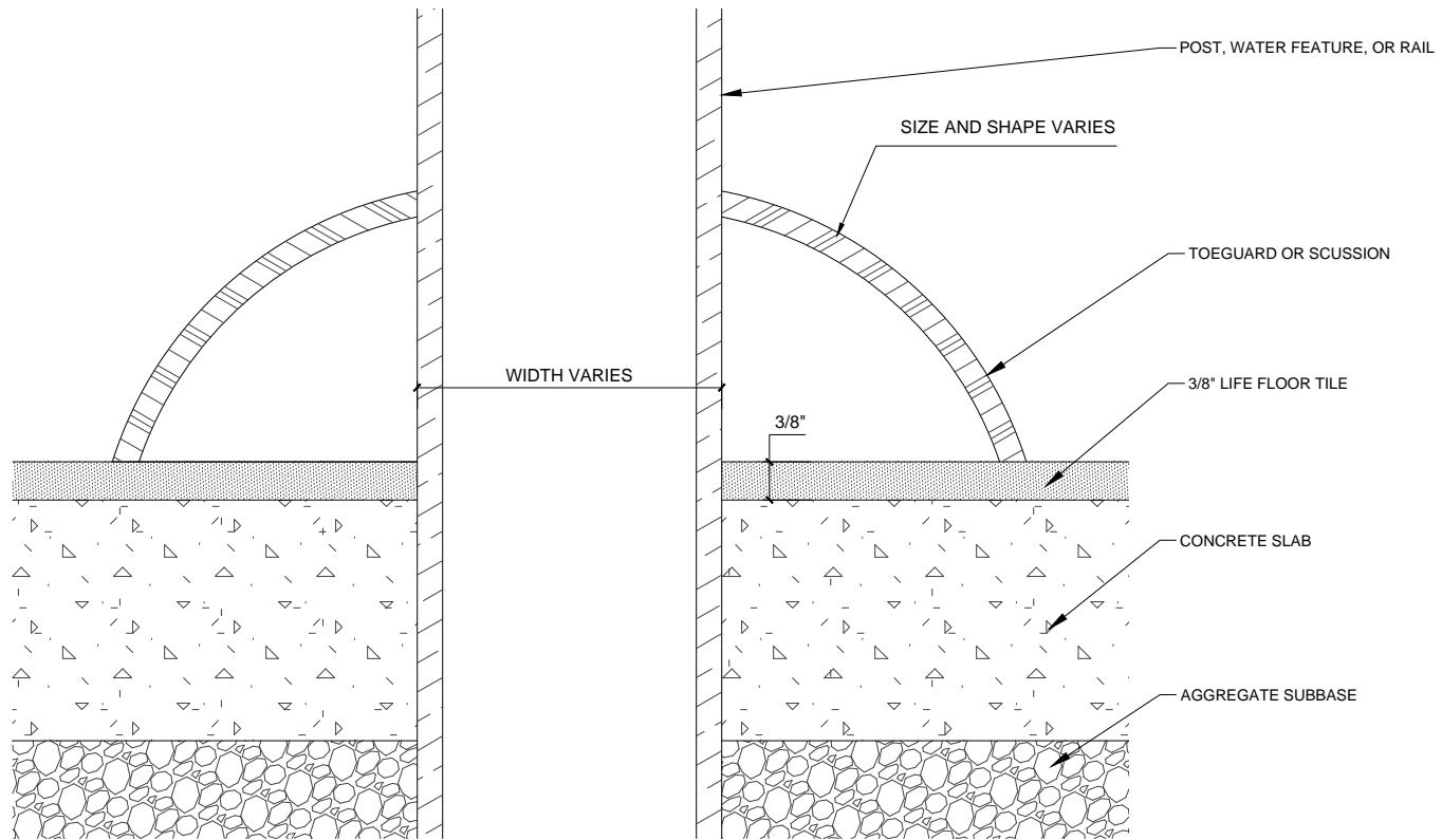
1 LIFE FLOOR APPLICATION WITH POST, WATER FEATURE, OR RAIL SCALE: 6" = 1'-0"
