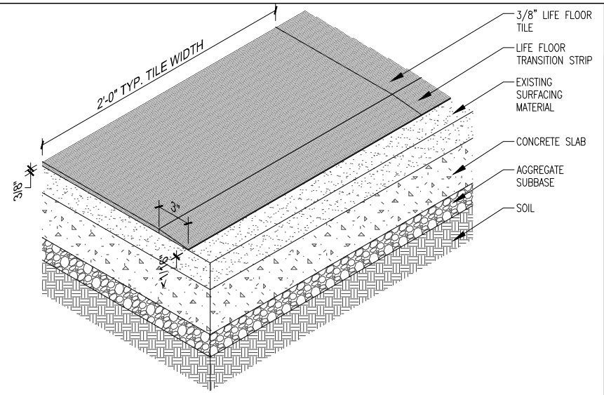
2 3/8" TILE WITH TRANSITION STRIP SCALE: 1" = 1'-0"
