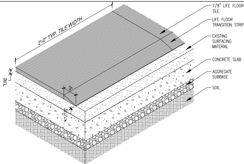
1 7/8" TILE WITH TRANSITION STRIP SCALE: 1" = 1'-0"
