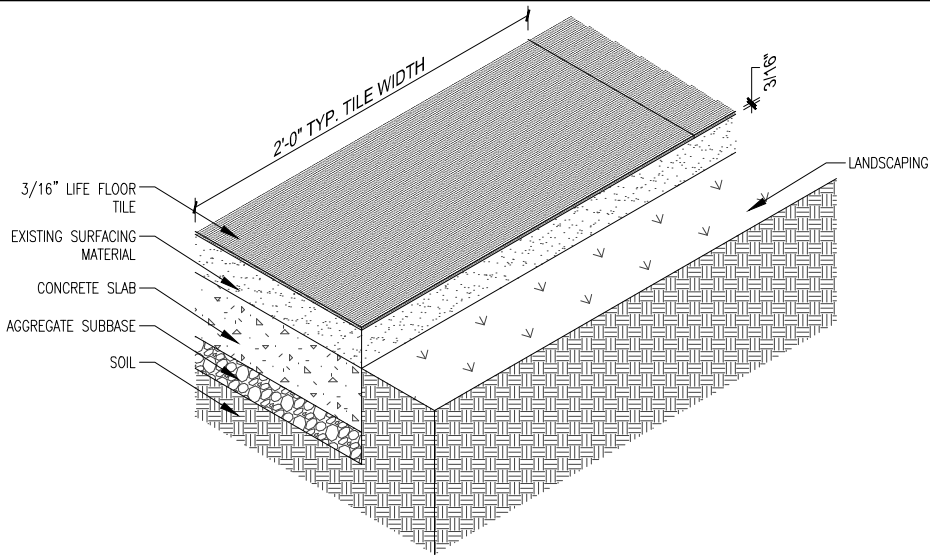
3 3/16" TILE FLUSH WITH EDGE OF EXISTING SURFACING MATERIAL SCALE: 1" = 1'-0"
